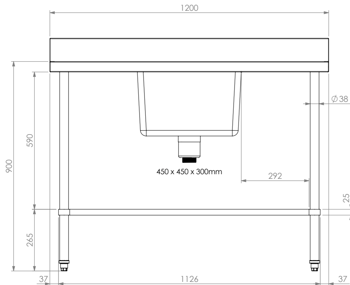
FRONT ELEVATION
